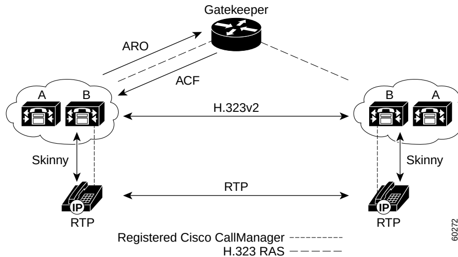
Figure 6-57 Call Flow Process for Inter-Cluster Topology
