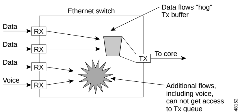
Figure 4-12 QoS Problem Areas (2 of 3)
