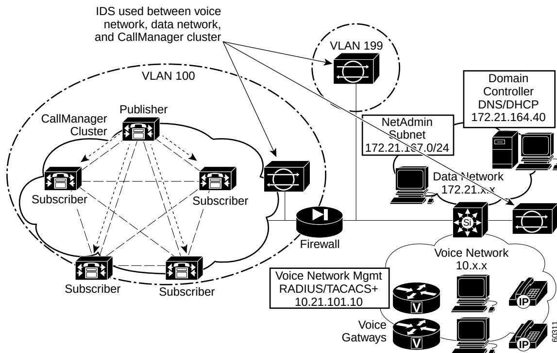
Figure 6-30 Network Intrusion Detection System
