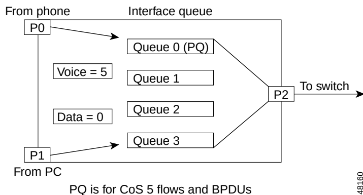
Figure 4-7 IP Phone Queueing
