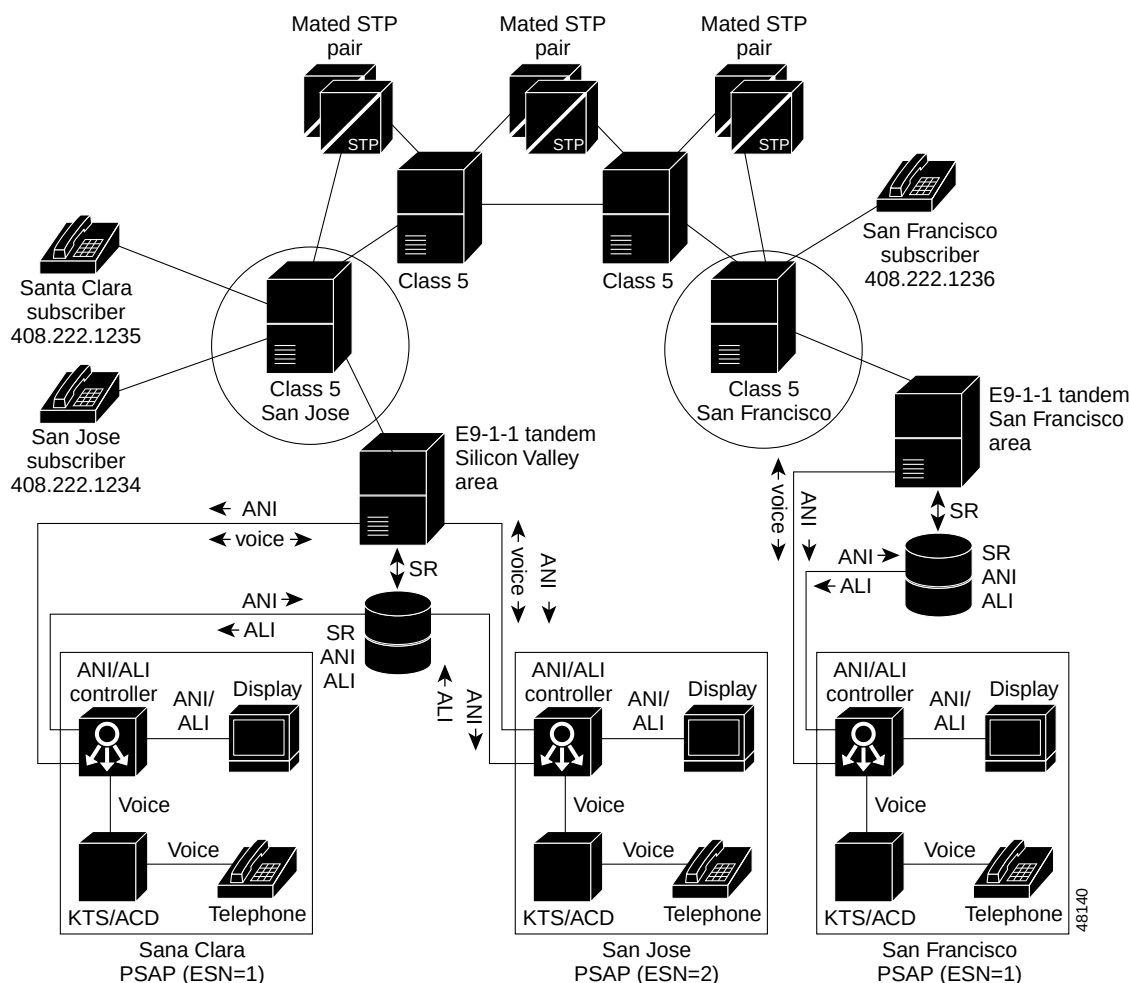
Figure 4-33 Typical E9-1-1 Network Topology
