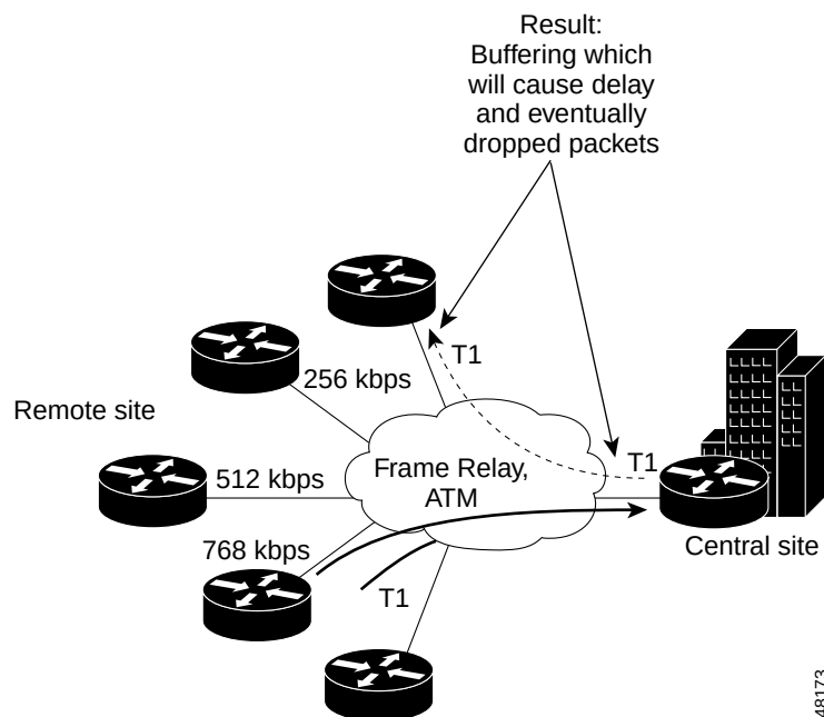
Figure 4-23 Traffic Shaping Scenario
