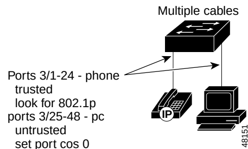
Figure 4-9 Catalyst 6000 Example with Multiple Cables
