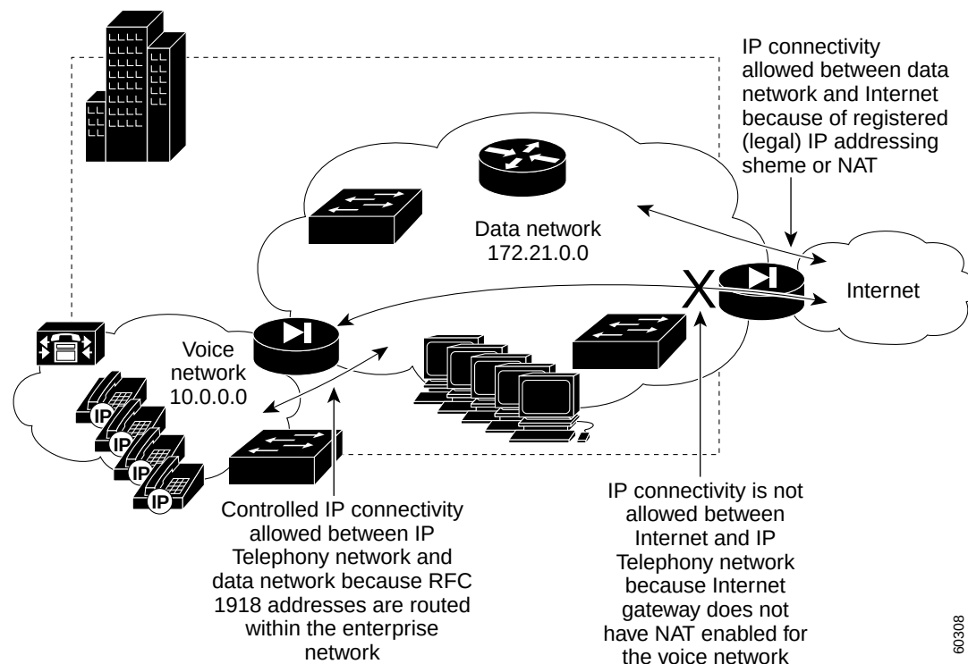
Figure 6-27 Logical IP Address Separation Using NAT
