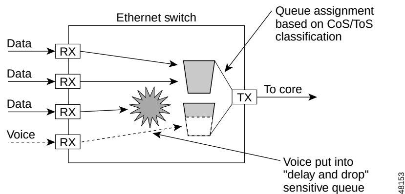
Figure 4-13 QoS Problem Areas (3 of 3)
