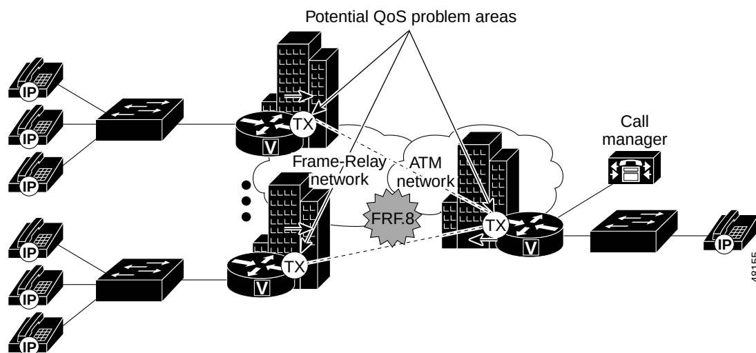
Figure 4-30 Frame Relay to ATM—QoS Problem Areas
