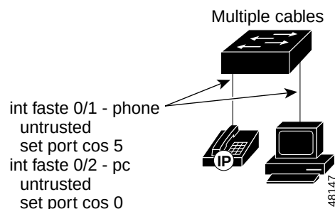
Figure 4-10 Catalyst 3500/2900 Example with Multiple Cables
